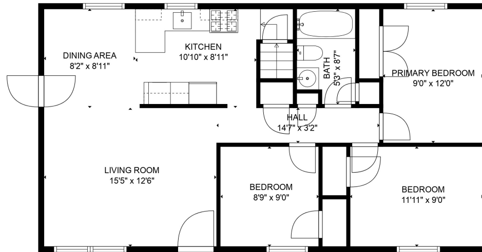
FLOOR 2
